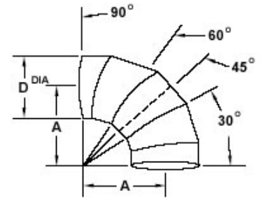
Elbows
