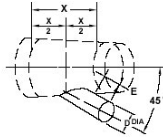
Laterals
