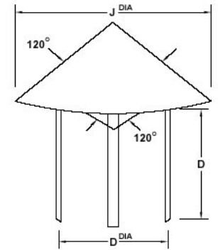
Rain Caps
